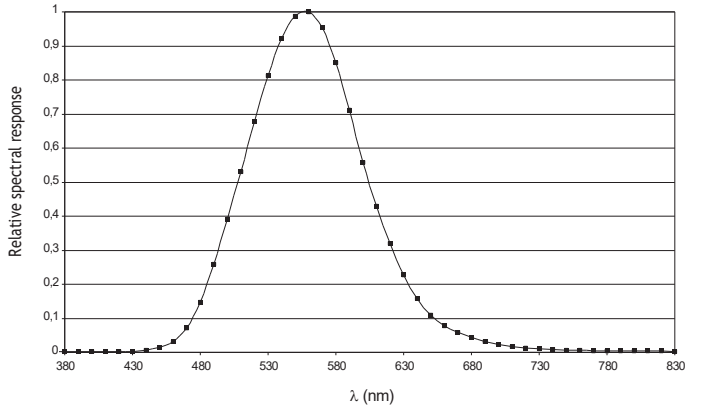
Typical response curve: LP471PHOT and LP471LUM2
