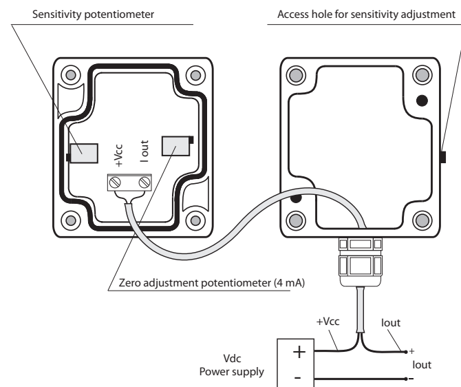
Fig. 2 - Connecting diagram with current output
